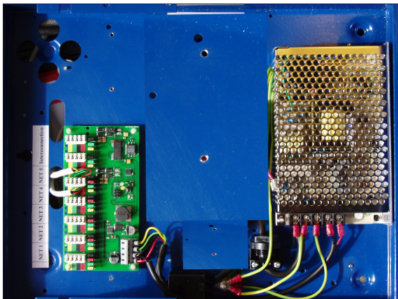
Repeater Box
