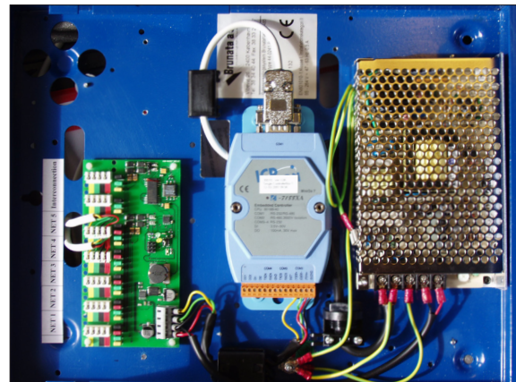
Controller Box
